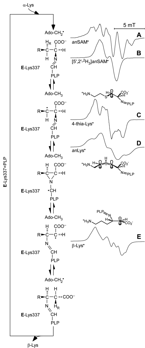
Figure 1. Reaction cycle for LAM with corresponding X-band (9 GHz) CW EPR spectra of intermediates or analogues of intermediates. Adapted from ref 31.
